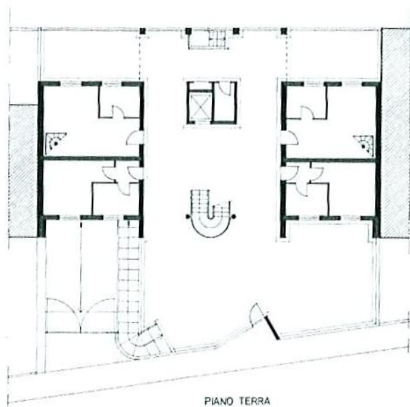
PIANO TERRA
